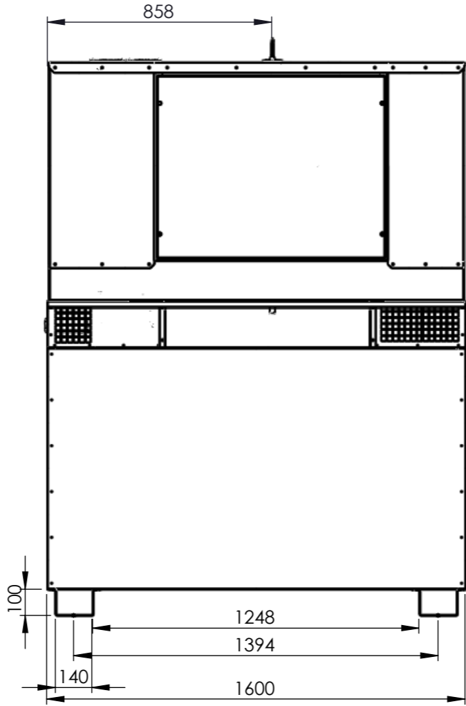
Floor mounting positions
